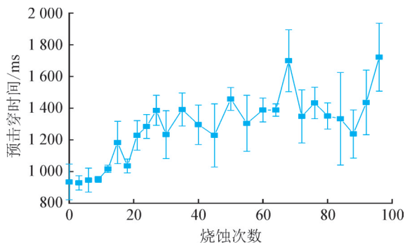
图17 电寿命退化过程中预击穿燃弧时间变化 Fig. 17 Variation of pre-arcing time during electrical endurance degradation
