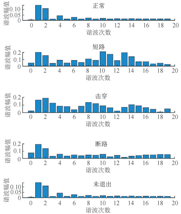
图9 合闸电阻投入期间谐波含量 Fig. 9 Harmonic content during switching of closing resistor
