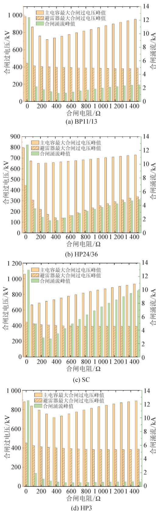
图6 滤波器合闸电阻阻值与合闸涌流及合闸过电压关系 Fig. 6 Relationship among closing resistor value, inrush current and switching overvoltage of filter banks
