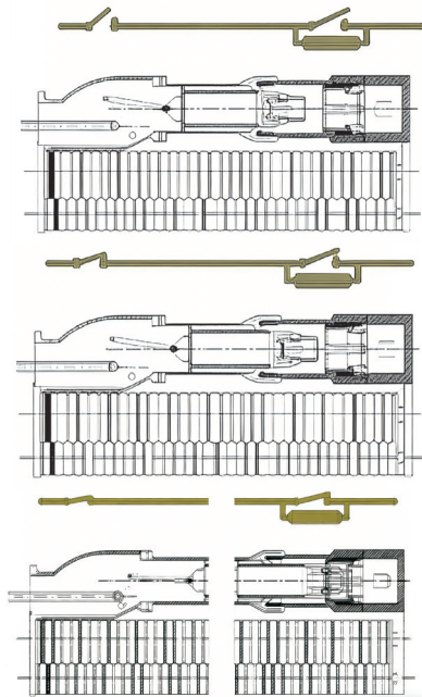
图4 合闸电阻型断路器关合动作过程 Fig. 4 Making operation process of circuit breaker with closing resistor
