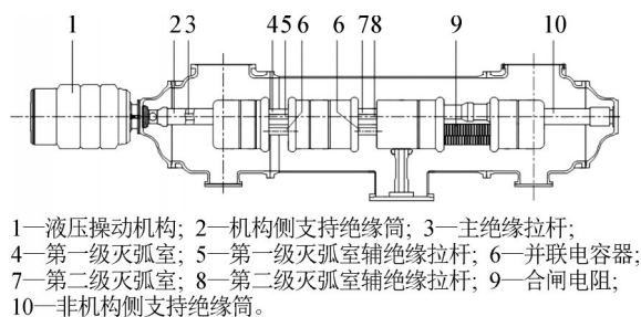
图3 合闸电阻型800 kV断路器结构 Fig. 3 Structure of 800 kV circuit breaker with closing resistor
