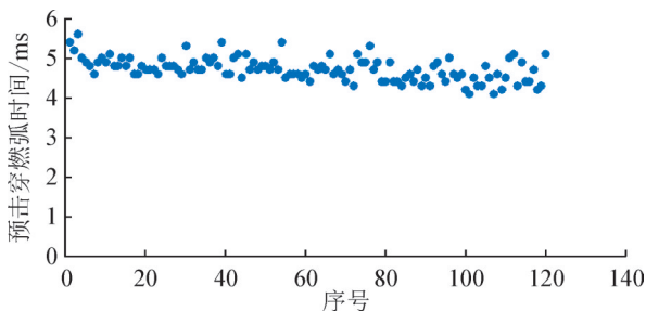
图16 BC2型式试验中关合预击穿燃弧时间 Fig. 16 Prestrike arcing time during making test of BC2 type test
