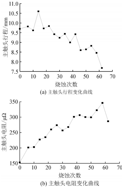
图12 主触头行程及电阻随烧蚀次数增加的变化趋势 Fig. 12 Variation trend of main contact travel and resistance with ablation cycles
