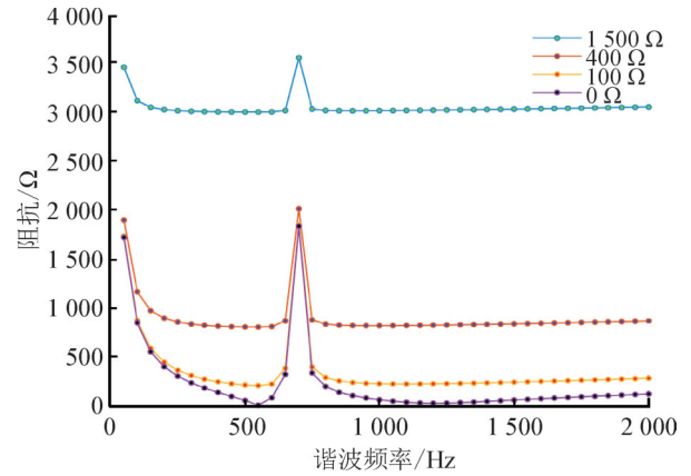
图8 不同合闸电阻值下的合闸电阻和滤波器组成支路的谐波阻抗 Fig. 8 Harmonic impedance of closing resistor and filter branch under different resistance values
