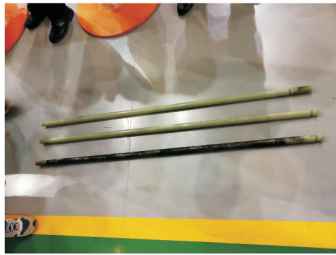
(c) 合闸电阻绝缘支撑杆熏黑
