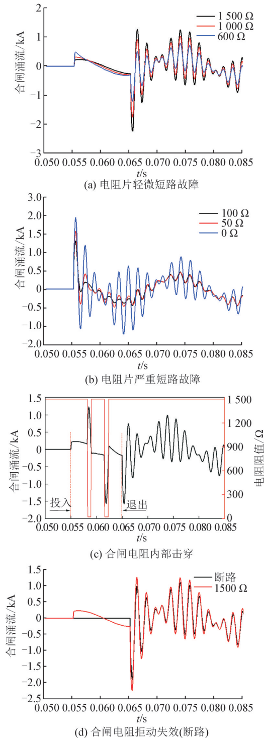
图7 合闸电阻投入阶段典型异常情况 Fig. 7 Typical abnormal condition during switching stage of closing resistor
