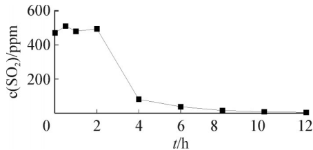
图15 吸附剂作用下的SO 2 浓度变化曲线 Fig. 15 Concentration variation curve of SO 2 under action of adsorbent
