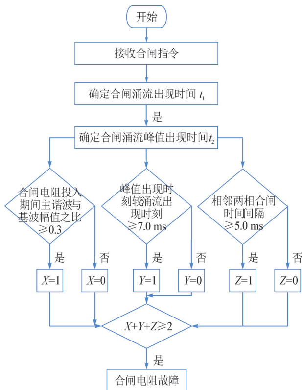
图 10 断路器合闸电阻故障诊断原理图 Fig. 10 Fault diagnosis principle diagram of closing resistor of circuit breaker
