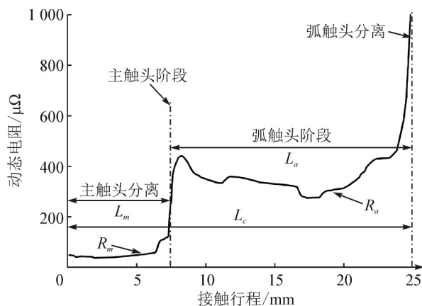
图 11 分闸过程的电阻-行程曲线 Fig. 11 Resistance-stroke curve during opening operation process
