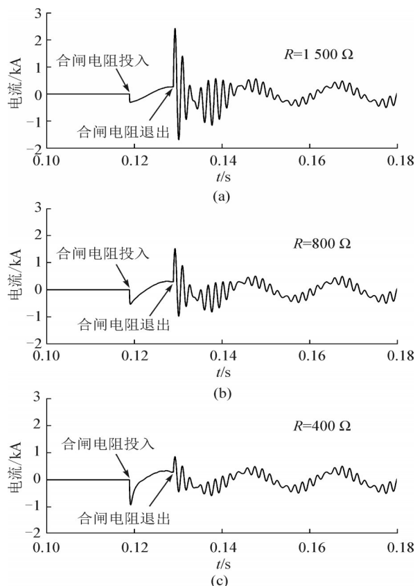
图5 装配不同阻值合闸电阻时合闸涌流波形 Fig. 5 Closing inrush current waveforms with assembly of closing resistors of different resistances
